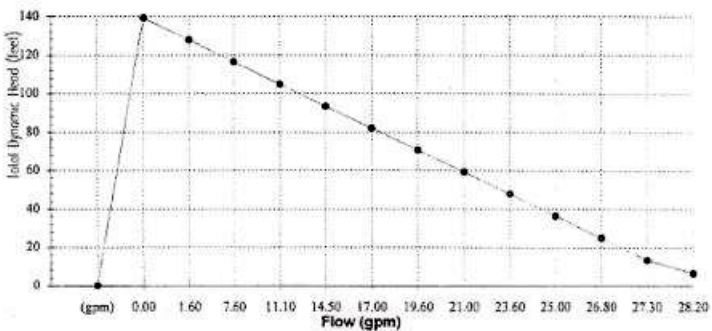
PB4 Pump Curve
